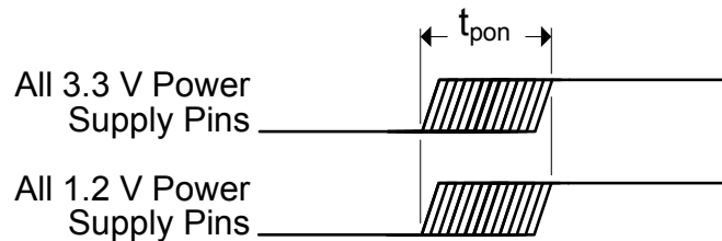
Figure 7.2 Power Sequence Timing
