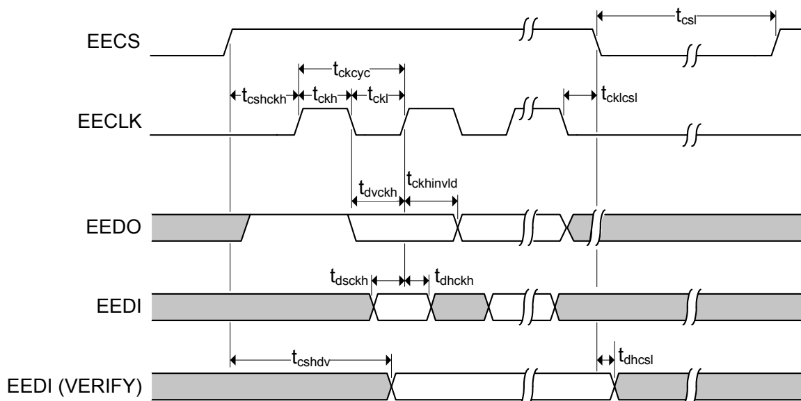
Figure 7.5 EEPROM Timing
